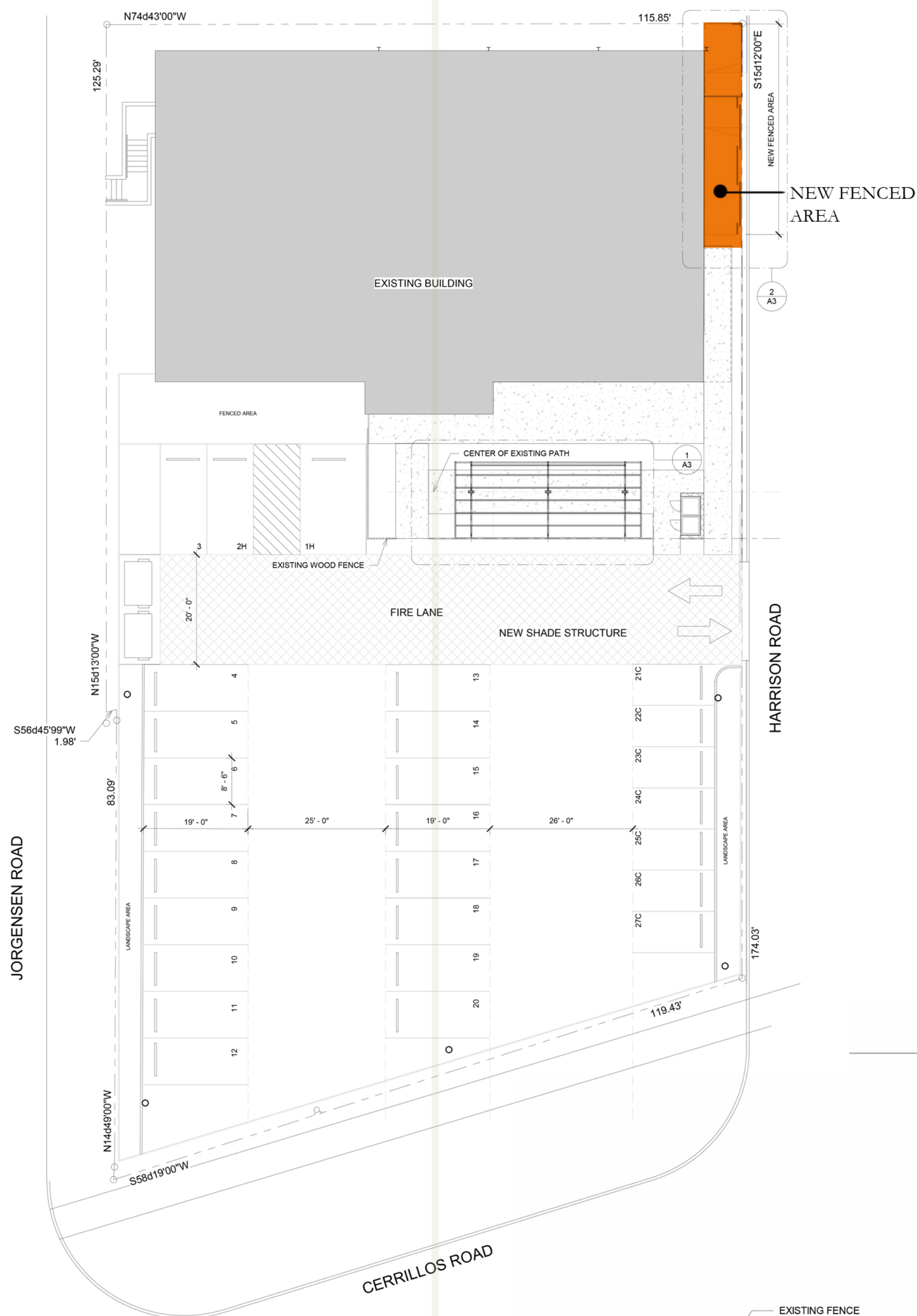
SITE PLAN
